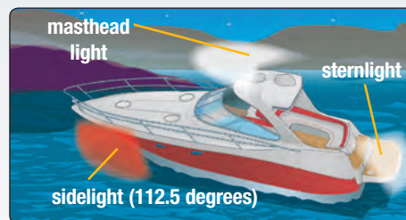
Navigation lights of a power-driven vessel with a masthead light, sternlight, and separate sidelights
